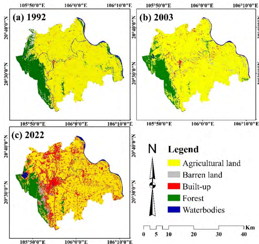
Fig. 3. Land use/land cover maps for Ha Nam province in 1992 (a), 2003 (b), and 2022 (c)
