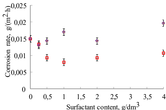
Fig. 10. Effect of surfactant content on the corrosion rate of steel substrate protected by acrylic coating in distilled water (within 30 minutes and temperature (25±2) °C)
